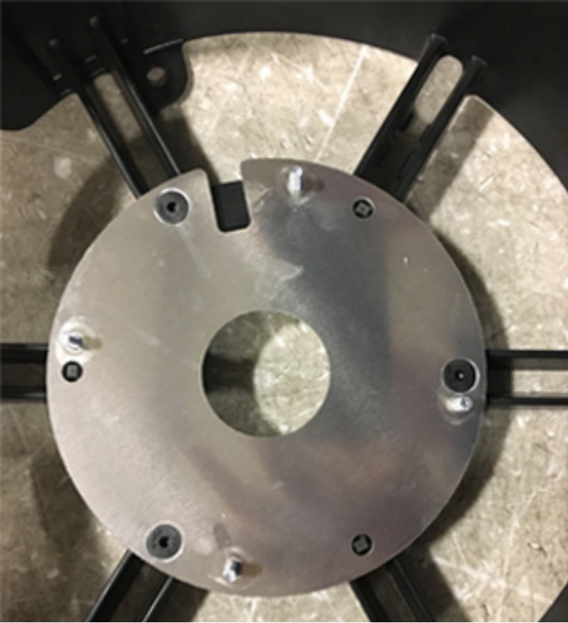
Remove old fan motor & secure plate to the shroud using the 3 socket screws
