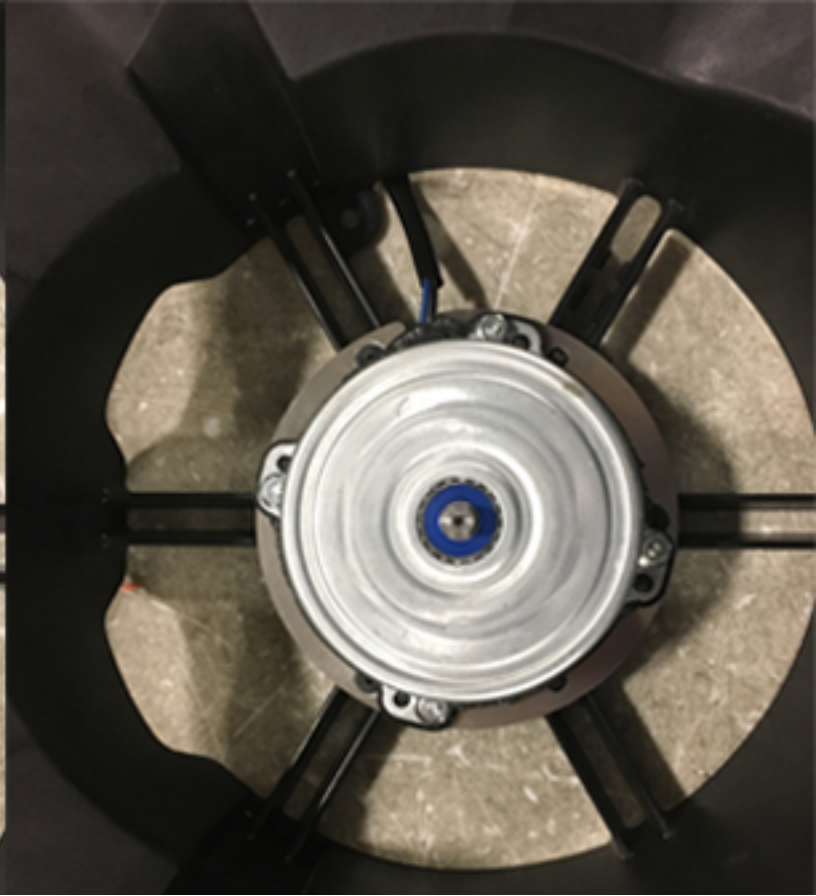
Set new SPAL fan motor on plate and secure with the 4 flange nuts
