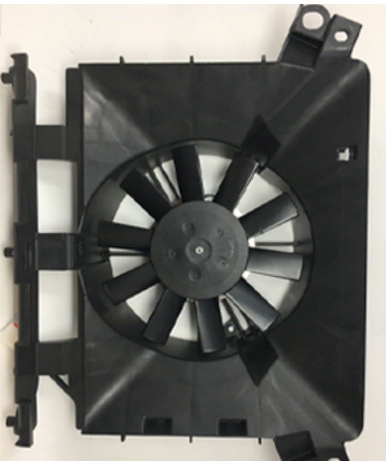
Set shaft pin then install fan blade and secure down with snap ring.
